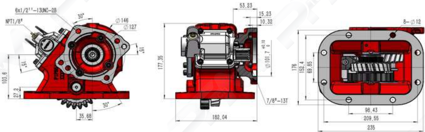
Dimension Drawing PTO489XQAHX-V3XK
