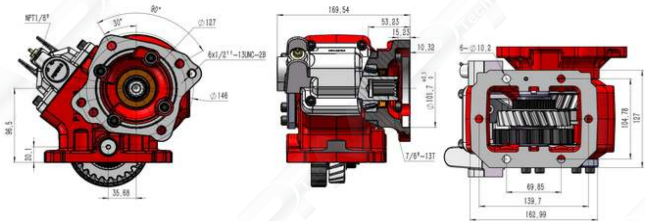
Dimension Drawing PTO442XQAHX-V3XK
