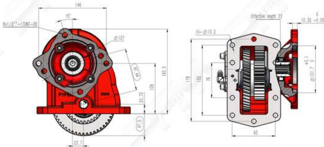
Dimension Drawing PTO267XGFJP-M5XK
