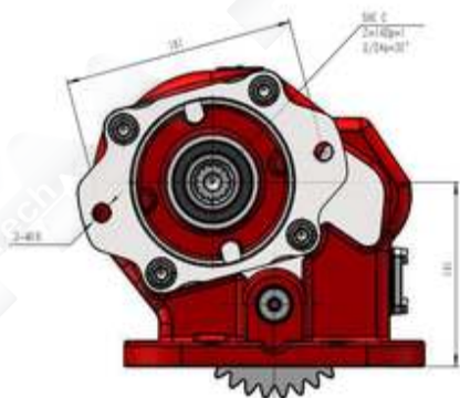
Dimension Drawing PTO852XGAKP-F6XS
