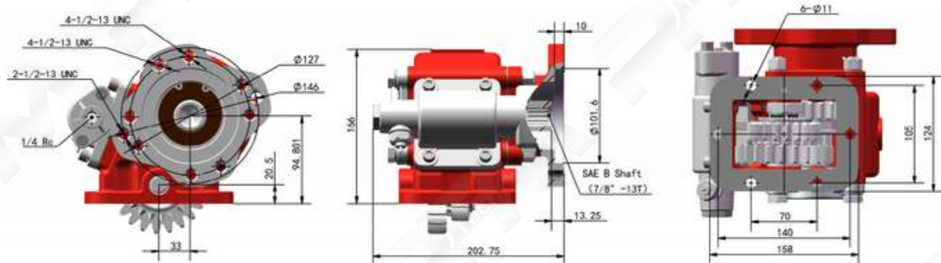
Dimension Drawing PTO1000XEN011RA
