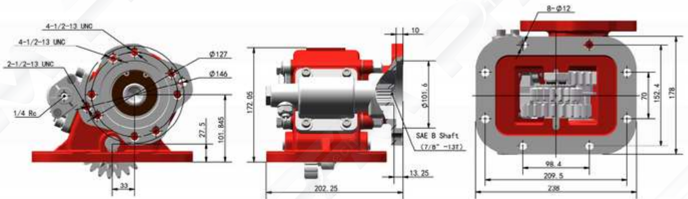
Dimension Drawing PTO2000XEN011RA
