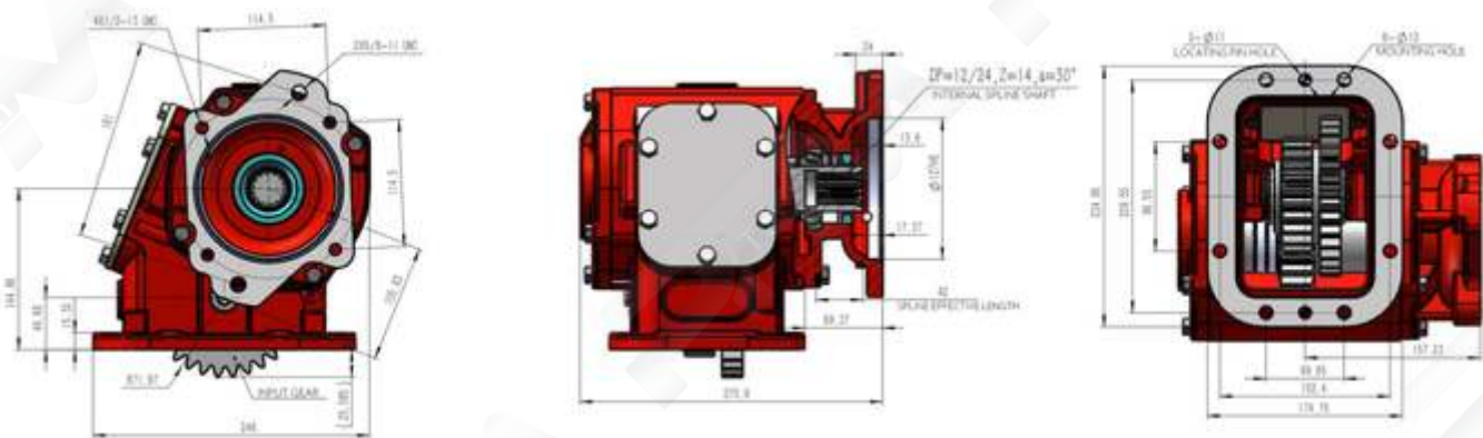
Dimension Drawing PTO880XBAKP-M4XS
